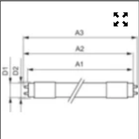
Dimension Drawing (with table) - Ecofit Main s LEDtube 600mm 8W 765 G
